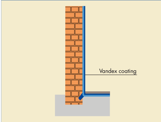
Basement waterproofing
